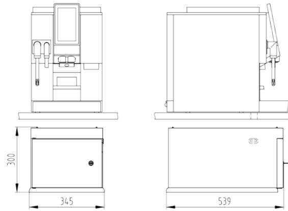
Under-machine cooling unit under the coffee machine
